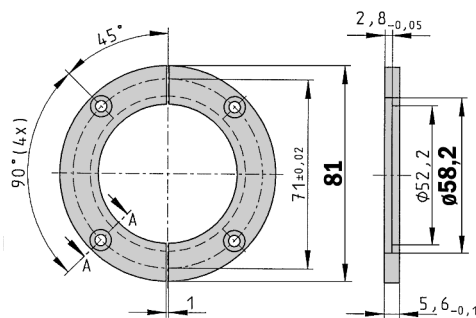
General tolerances according DIN ISO 2768-mk
