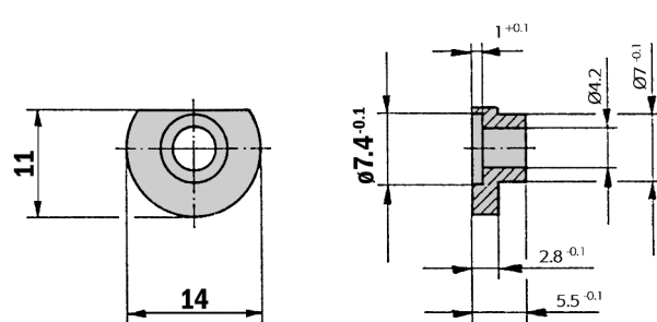
General tolerances according DIN ISO 2768-mk
